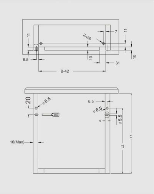
抽屉尺寸及打孔图 Drawer Size And Drilling Diagram
