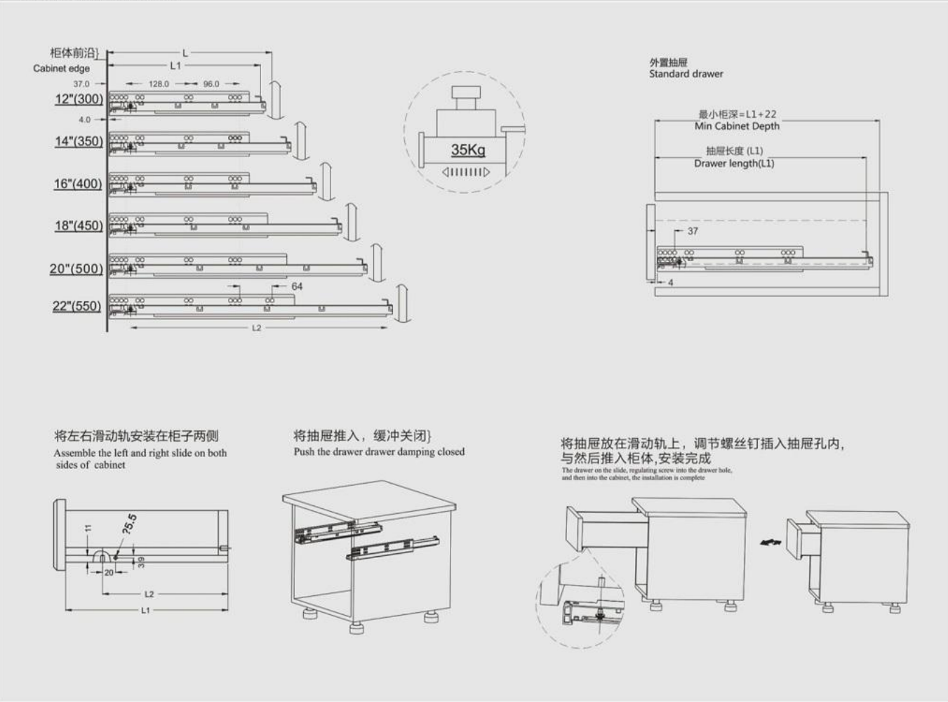
安装孔位图 Hole Pattern For Installation
