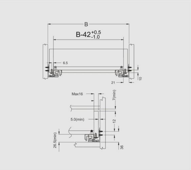
安装孔位图 Hole Pattern For Installation
